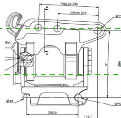
XT7 Weight: ≈152 kg Building Height: 394 mm
