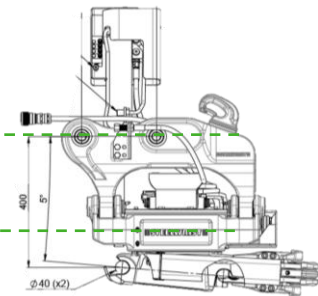
X07 Weight: ≈190 kg Building Height: 400 mm
