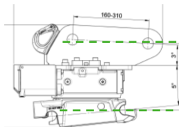
XR7 Weight: ≈120 kg Building Height: 272 mm
